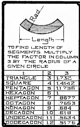
FIG. 211. TABLE FOR SEGMENTAL WORK ON TRIMMER.
